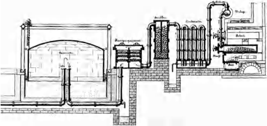
Gasfabriek, schema fabricage steenkolen gas in 1860
